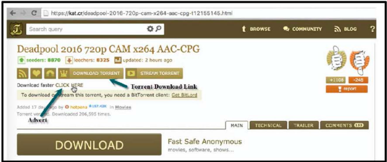
Figure 3: Undercover Advertisement
